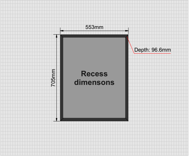
Recess dimensions: 553mm Width x 705mm height x 96.6mm Depth
