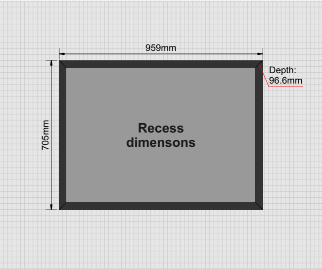
Recess dimensions: 959mm Width x 705mm height x 96.6mm Depth
